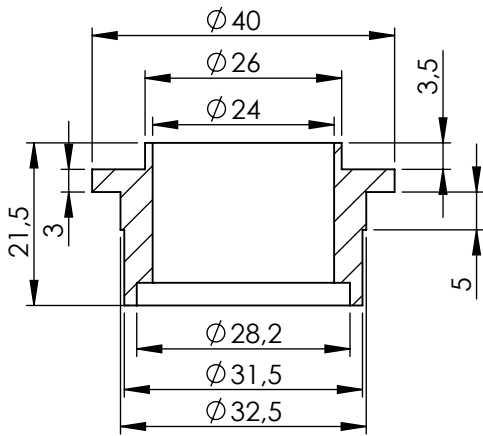
Bushing s.s cod.206283
